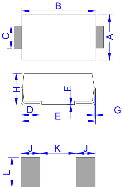
DO-214AA (SMB)
