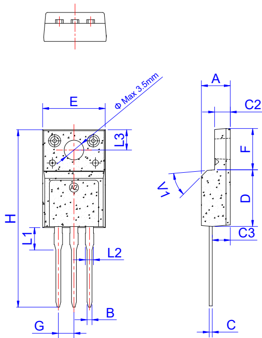
TO-220FA
